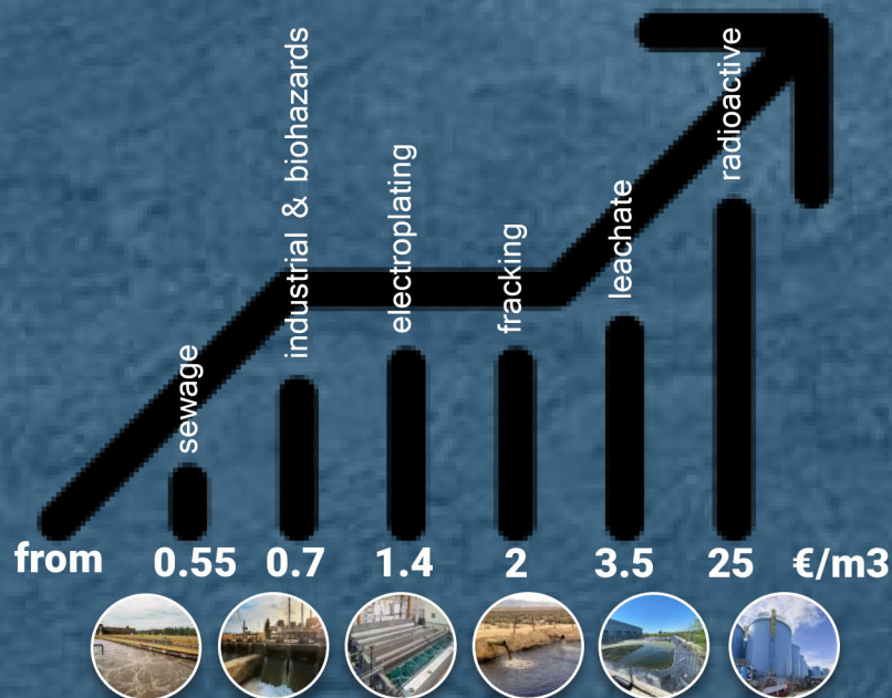
OPERATIONAL COSTS FOR TREATMENT OF SOME PARTICULAR TYPES OF LIQUID WASTE
