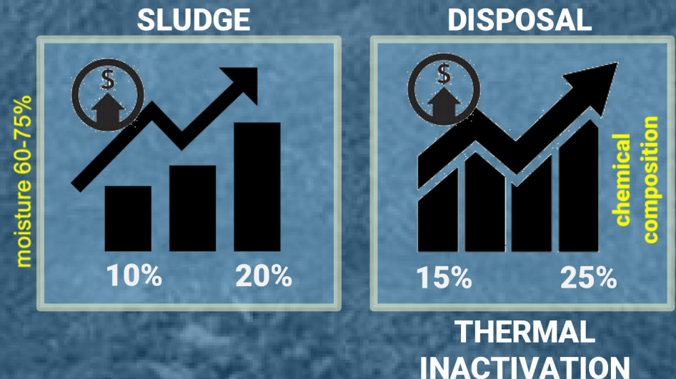
TYPICAL EXPENSES FOR SLUDGE THICKENING AND DISPOSAL AS PERCENT FROM THE TOTAL TREATMENT COSTS
